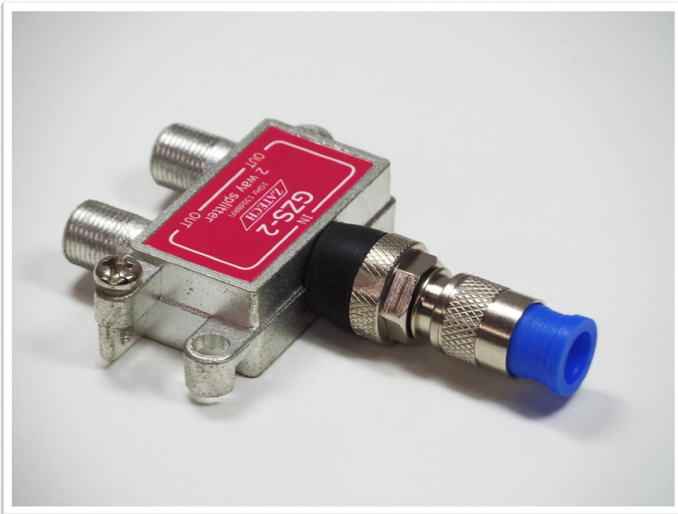
Conector F-macho
