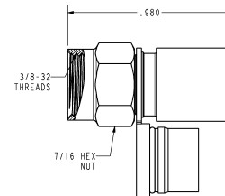
Fig. C Connector & Sleeve
